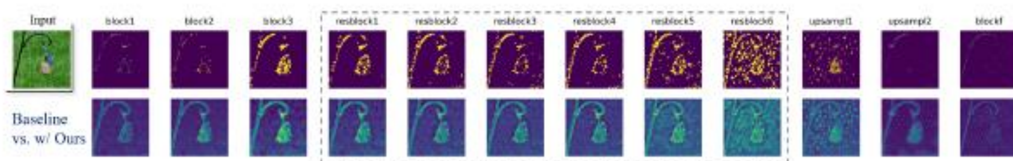
Block-wise perturbation generation progression
